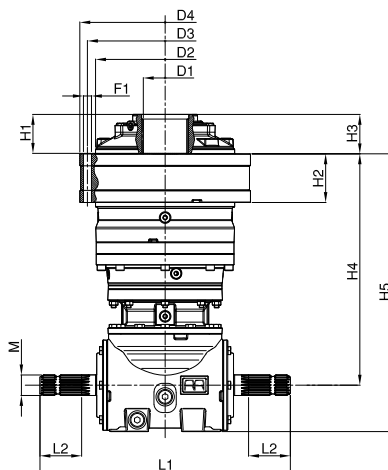
OUTPUT FLANGE INTERFACE
