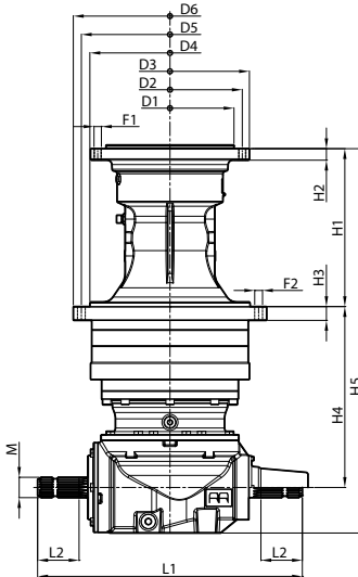
OUTPUT FLANGE INTERFACE
